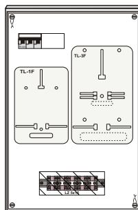
ZPP-60
