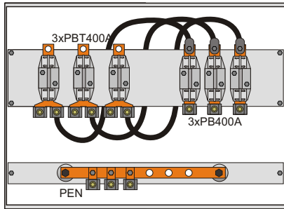
ZK-3a 400A
