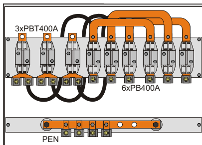
ZK-3e/RB 400A
