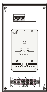
ZPP-3/60
